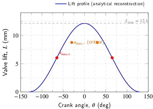
Figure 3: Schematic position of the two critical points of the cam profile of the AP 1.8 high-performance head: positive-acceleration peak ( a_{max,+} = 14\,544 \text{ m s}^{-2} at L_{+} = 6.04 \text{ mm} ) and deceleration peak ( a_{max,-} = 20\,362 \text{ m s}^{-2} at L_{-} = 8.747 \text{ mm} ). The full lift profile is generated from the cam sizing of the intake valve.
